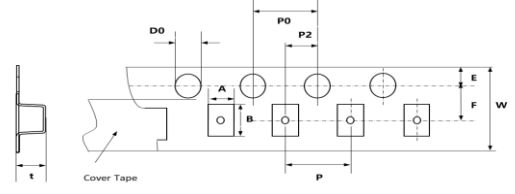
Fig. 5-2:0603,0805,1206,1210, 2220 (Plastic tape)
