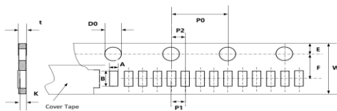
Fig. 5-5:0201 (Paper tape/ 1mm pitch)
