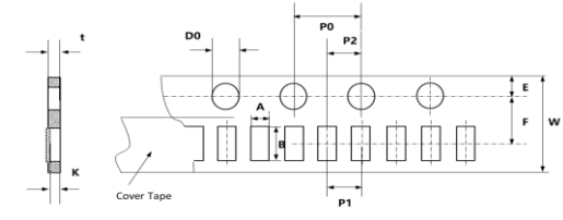
Fig. 5-4:0201 (Paper tape/ 2mm pitch)
