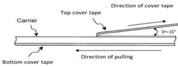
Fig.8 Cover tape peel-off force
