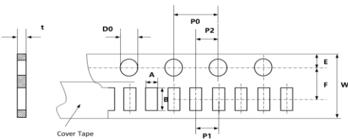
Fig. 5-3:0402 (Paper tape/ 2mm pitch)
