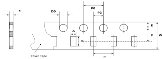
Fig. 5-1:0603,0805,1206,1210 (Paper tape)
